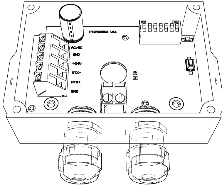
Figure 1. View of the printed circuit of the HCC-04-Modbus transducer
