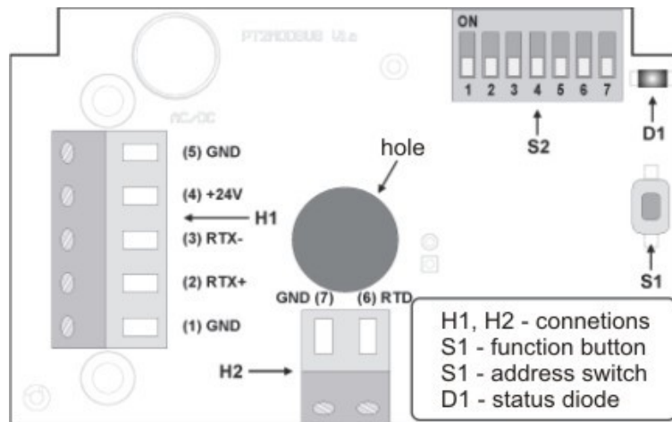
Figure 2. Description of the pinouts of the HCC-04-Modbus transducer
